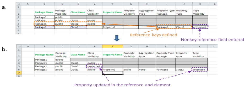
Figure 2.30: Values Entered in Nonkey Reference Fields with Key Reference Fields Defined
