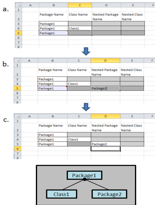
Figure 2.16: Defining Package2
